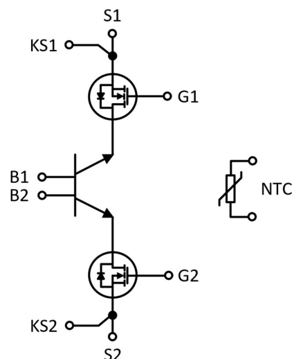
Device Circuit Symbol
