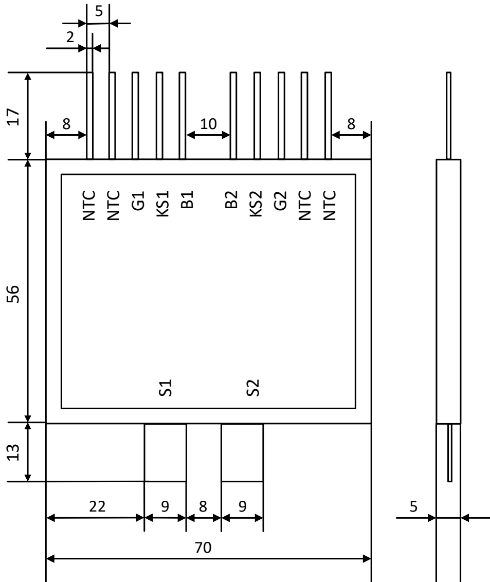
Figure 4: Mechanical outline of SymCool™ Power Module
